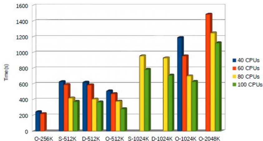
Figure 3.3: PaCE timing results on the benchmarks on different clusters 40, 60, 80, 100 CPUs
